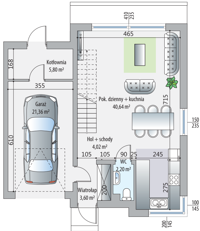
Parter -70.04 m 2
